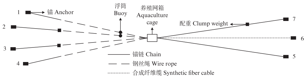
图1 养殖网箱锚泊系统组合 Fig.1 Combination of aquaculture cage mooring system
